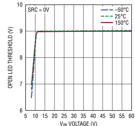
Open LED Threshold Rising vs V_{\text{IN}} , Temperature for V_{\text{OTH}}[1:0] = 01
